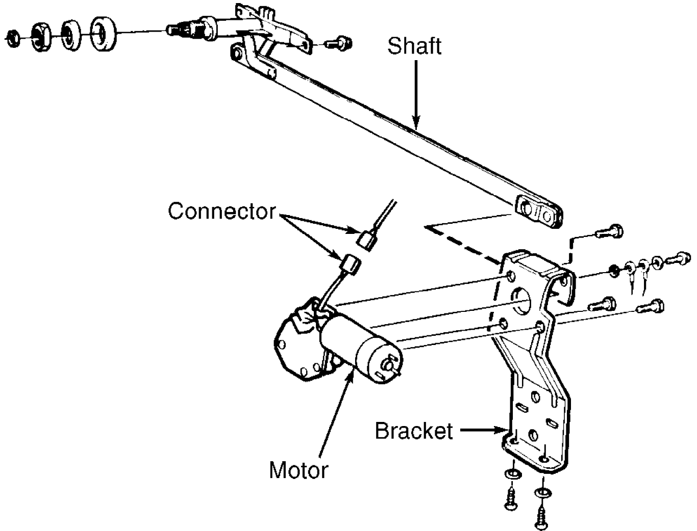
Fig. 4: Removing Rear Wiper Motor Courtesy of Volvo Cars of North America
