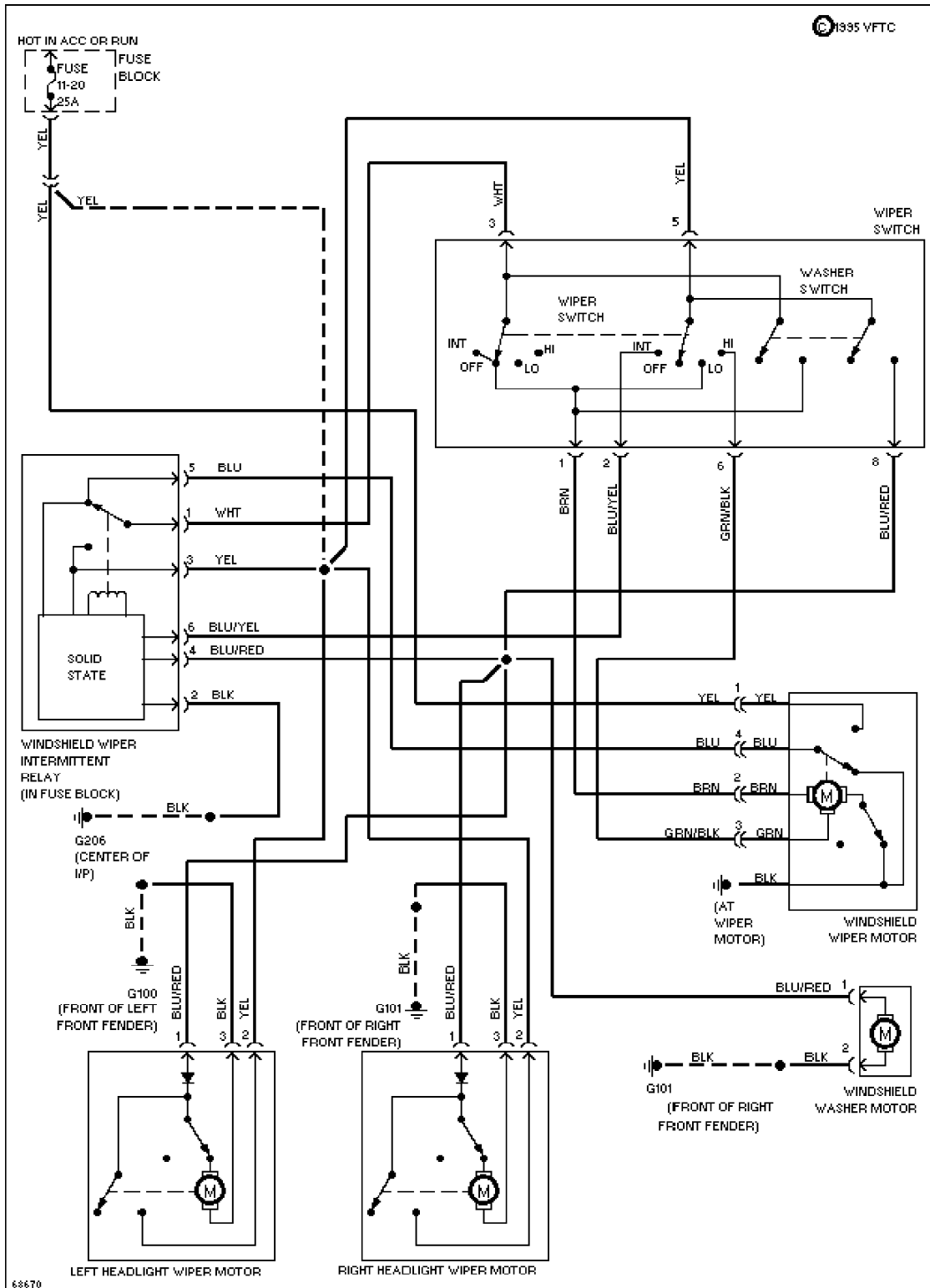
Fig. 5: Windshield/Headlt. Wiper/Washer System Wiring Diagram (1960)
