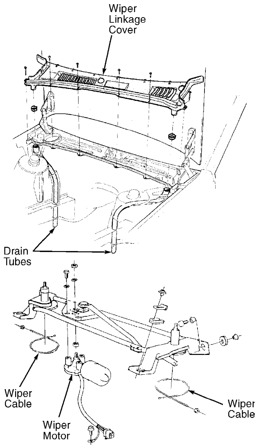
98J07464 Fig. 2: Removing Front Wiper Motor (960) Courtesy of Volvo Cars of North America
