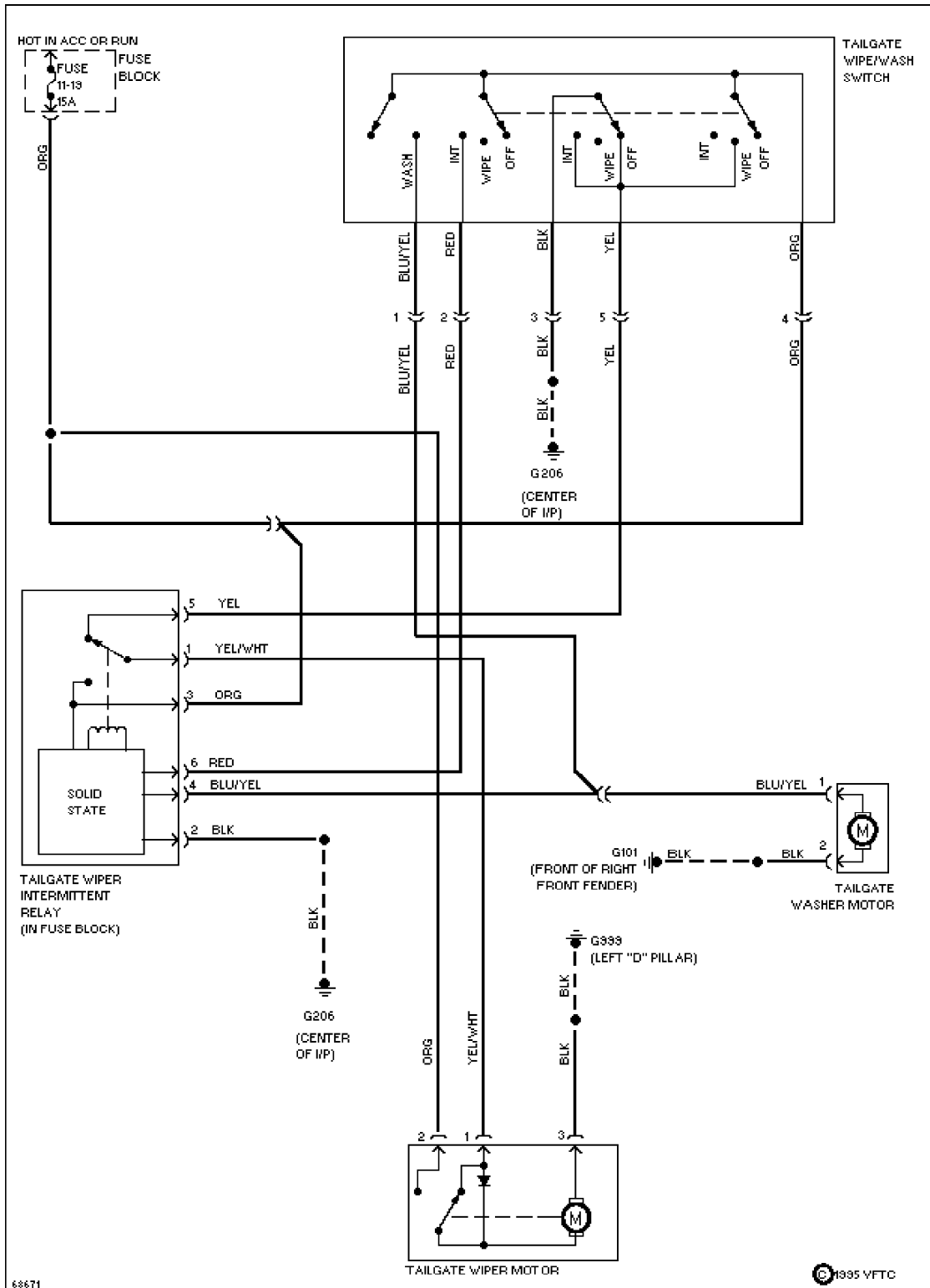
Fig. 6: Rear Wiper/Washer System Wiring Diagram (1960)
