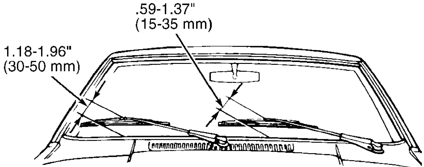
Fig. 1: Adjusting Wiper Arms (960) Courtesy of Volvo Cars of North America
