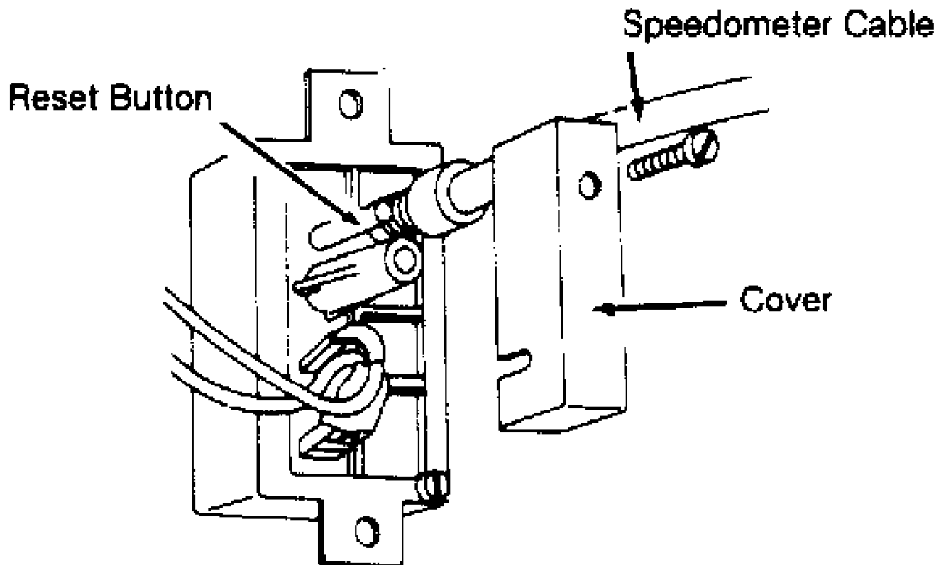
Fig. 1: Resetting Mileage Counter Courtesy of Volvo Cars of North America.
