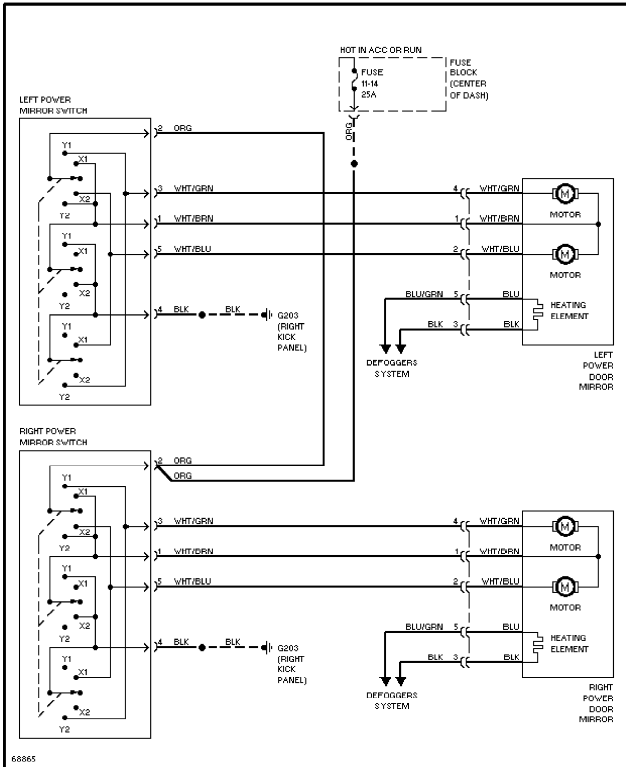
Fig. 5: Power Mirrors Wiring Diagram (960)
