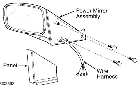
Fig. 4: Removing Power Mirror Assembly (960) Courtesy of Volvo Cars of North America
