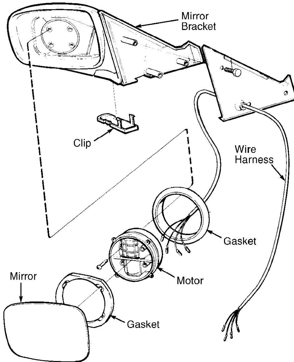
Fig. 1: Exploded View Of Power Mirror Assembly (960) Courtesy of Volvo Cars of North America
